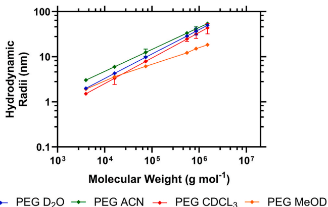
Fig. 4. Viscosity corrected hydrodynamic radii vs molar mass of PEG samples analysed in deuterated ACN (green, \alpha = 0.46 ), D 2 O (blue, \alpha = 0.62 ), CDCl 3 (red, \alpha = 0.70 ) and MeOD (orange, \alpha = 0.52 ). (For interpretation of the references to colour in this figure legend, the reader is referred to the Web version of this article.)
